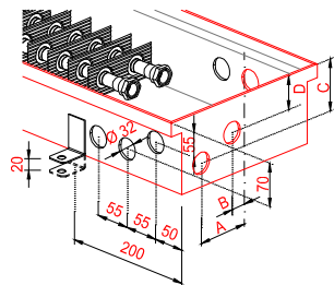
KORAFLEX FV 11/28 A=80, B=20, C=74, D=57 11/34 A=79, B=10, C=70, D=62 11/42 A=120, B=31, C=70, D=54
